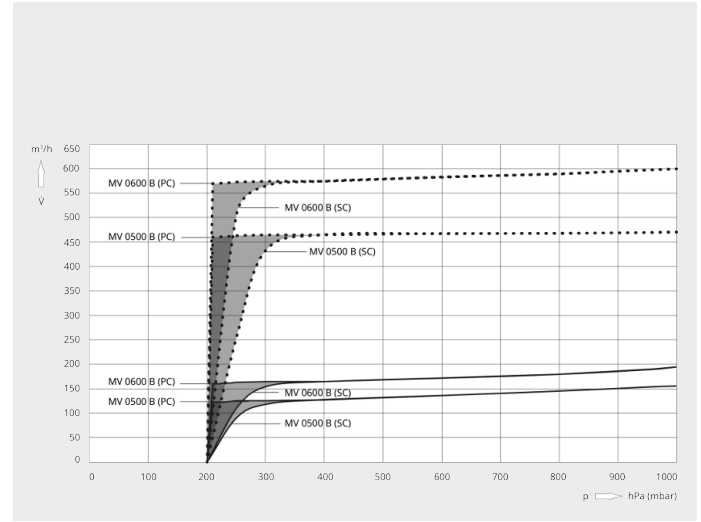
Pumping speed
